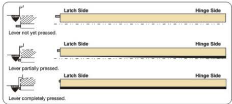
View of Cam installed on exterior latch side of door jamb (Chaukhat).
